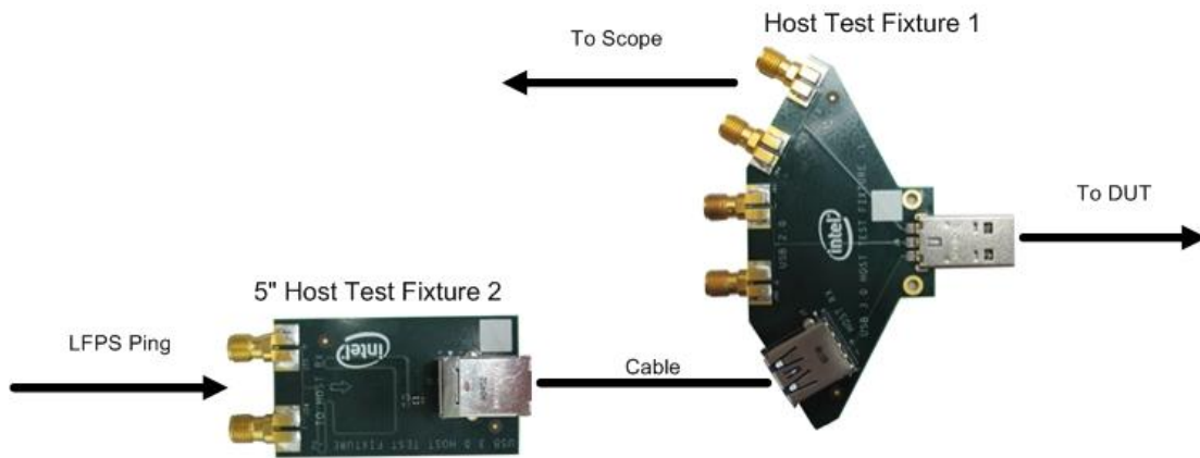
Figure 6: Host Tx Test Topology
