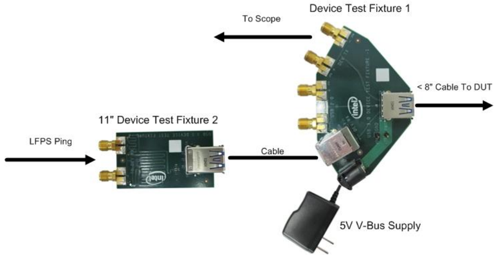
Figure 5: Device Tx Test Topology
