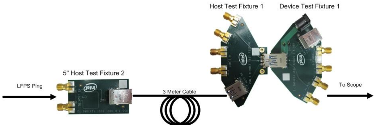
Figure 2: Host Rx Calibration Topology
