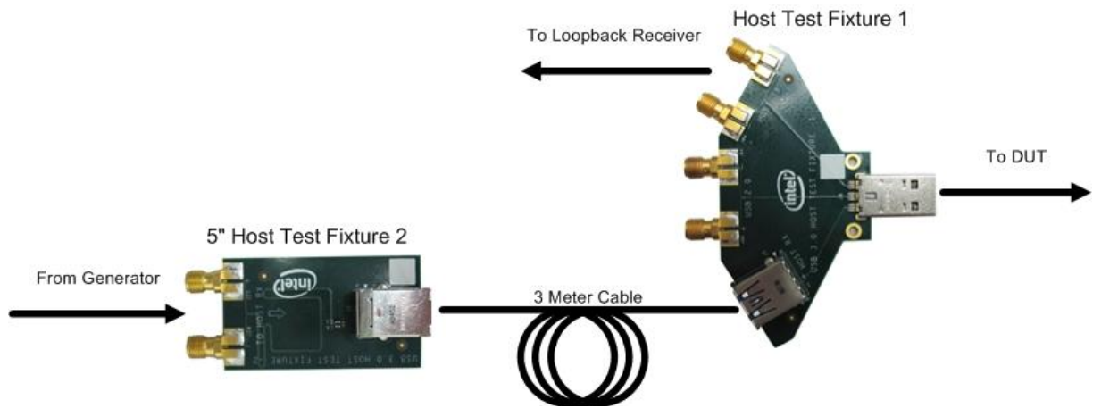
Figure 3: Host Rx Test Topology
