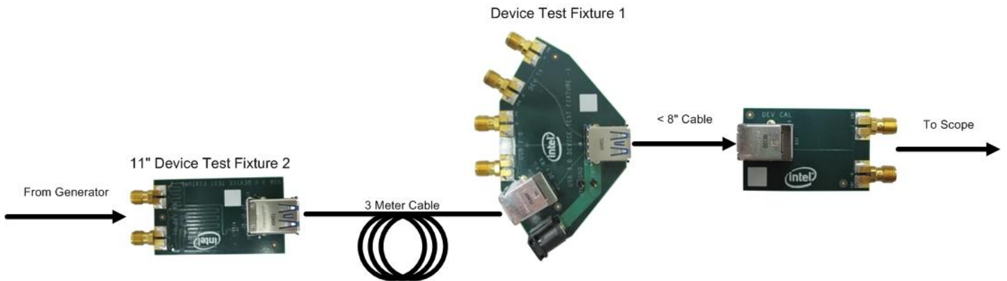
Figure 1: Device Rx Calibration Topology
