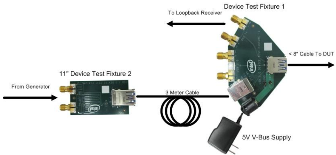
Figure 4: Device Rx Test Topology
